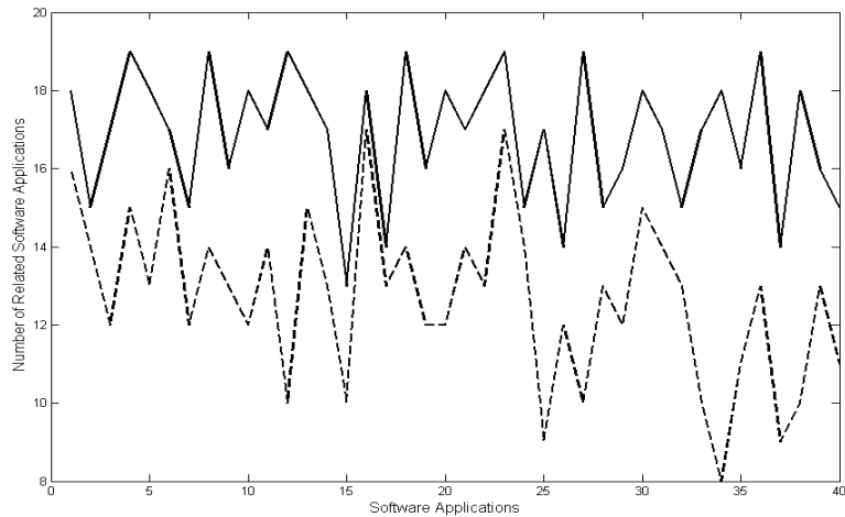
Fig. 3. The comparison between ECSC (solid line) and the original method (dashed line) over 40 software applications. The vertical axis shows the number of software applications returned that are shared with the results produced by human users.
